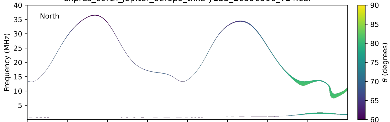
expres_earth_jupiter_europa_txka-y235_20390306_v14.cdf
