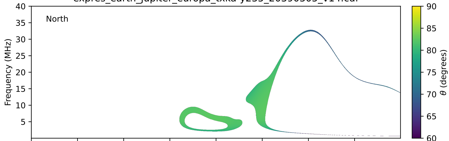
expres_earth_jupiter_europa_txka-y235_20390305_v14.cdf
