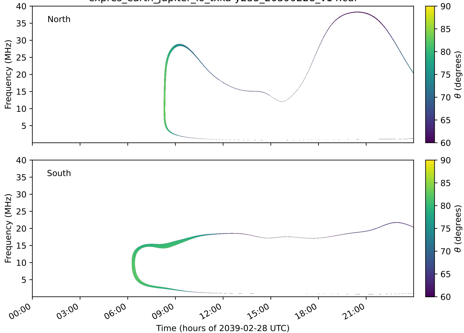
expres_earth_jupiter_io_txka-y235_20390228_v14.cdf
