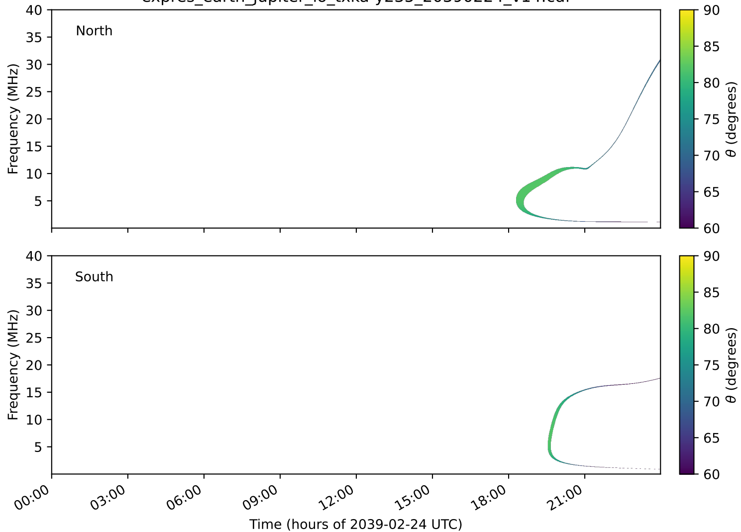
expres_earth_jupiter_io_txka-y235_20390224_v14.cdf
