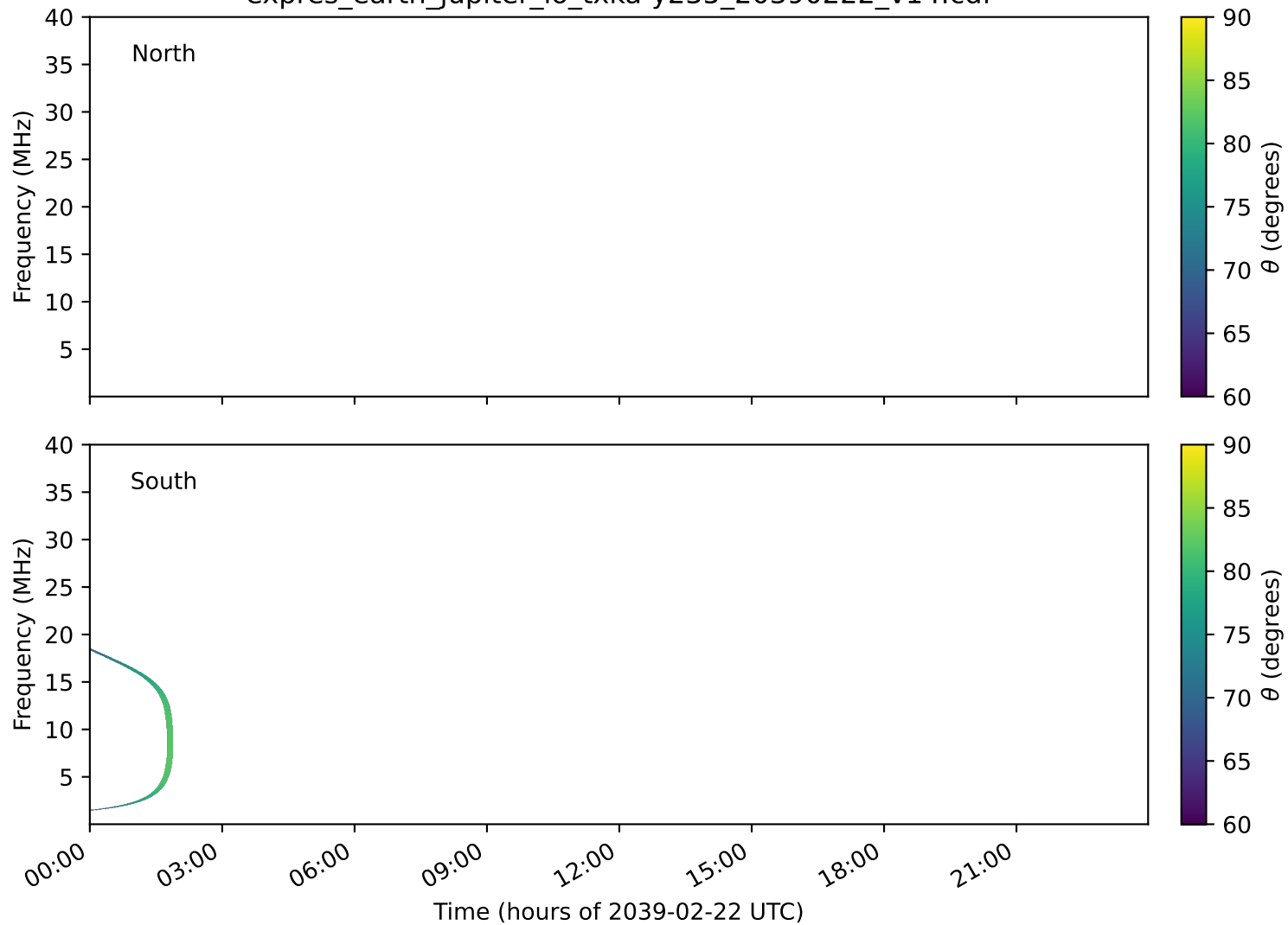
expres_earth_jupiter_io_txka-y235_20390222_v14.cdf
