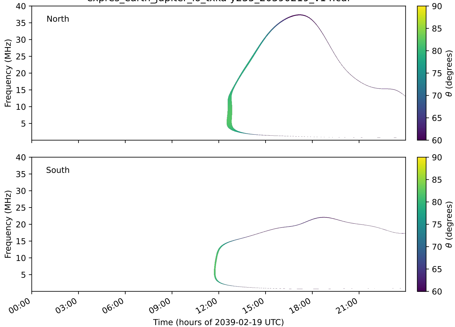
expres_earth_jupiter_io_txka-y235_20390219_v14.cdf
