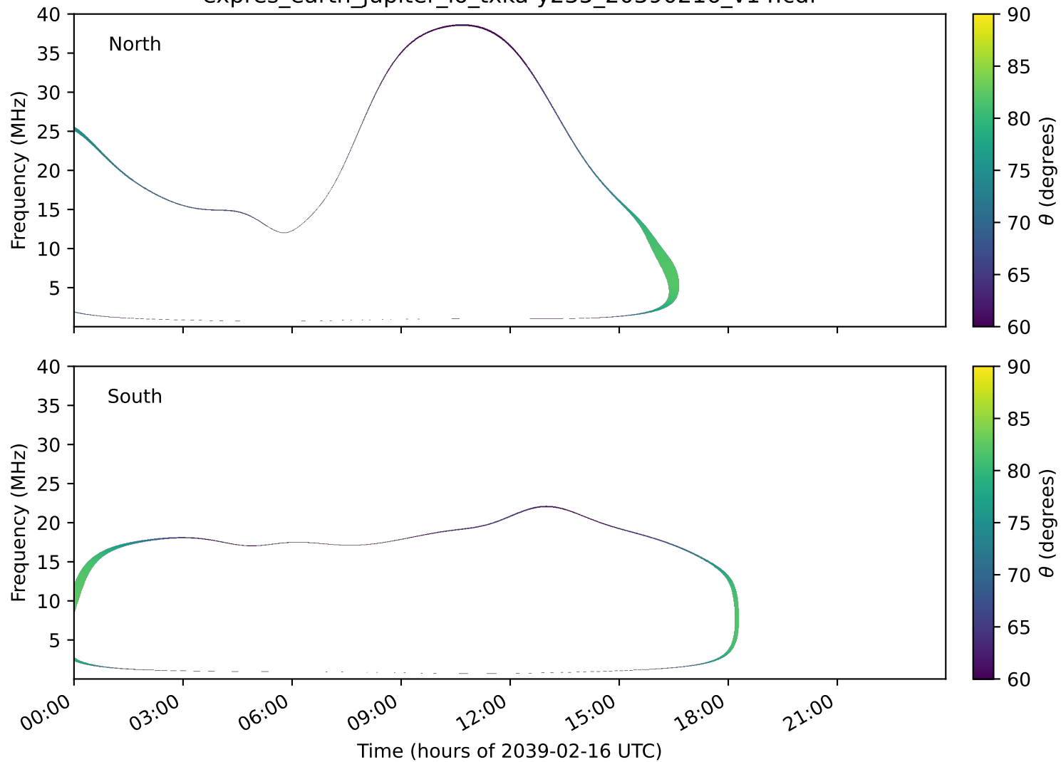
expres_earth_jupiter_io_txka-y235_20390216_v14.cdf
