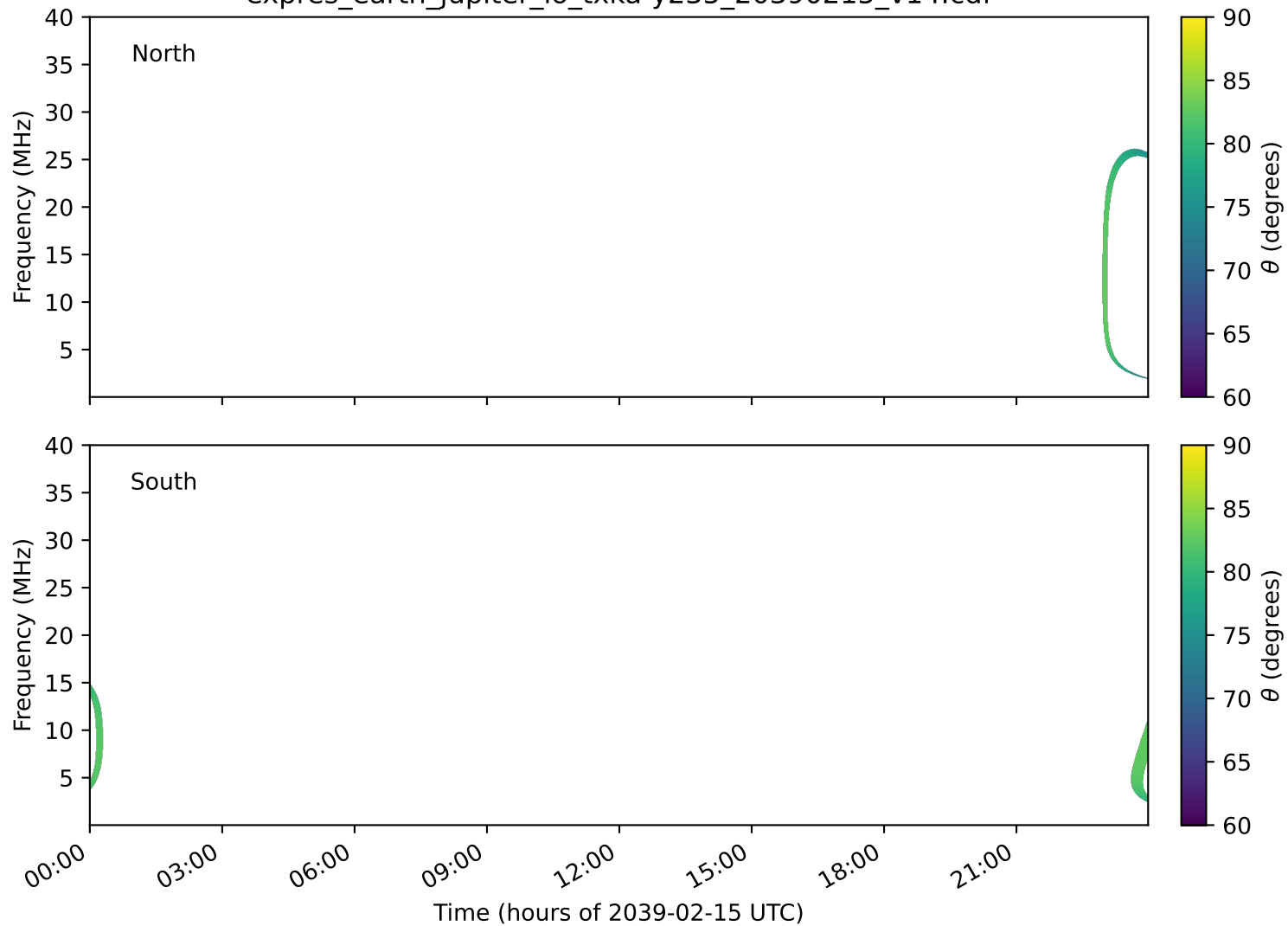
expres_earth_jupiter_io_txka-y235_20390215_v14.cdf
