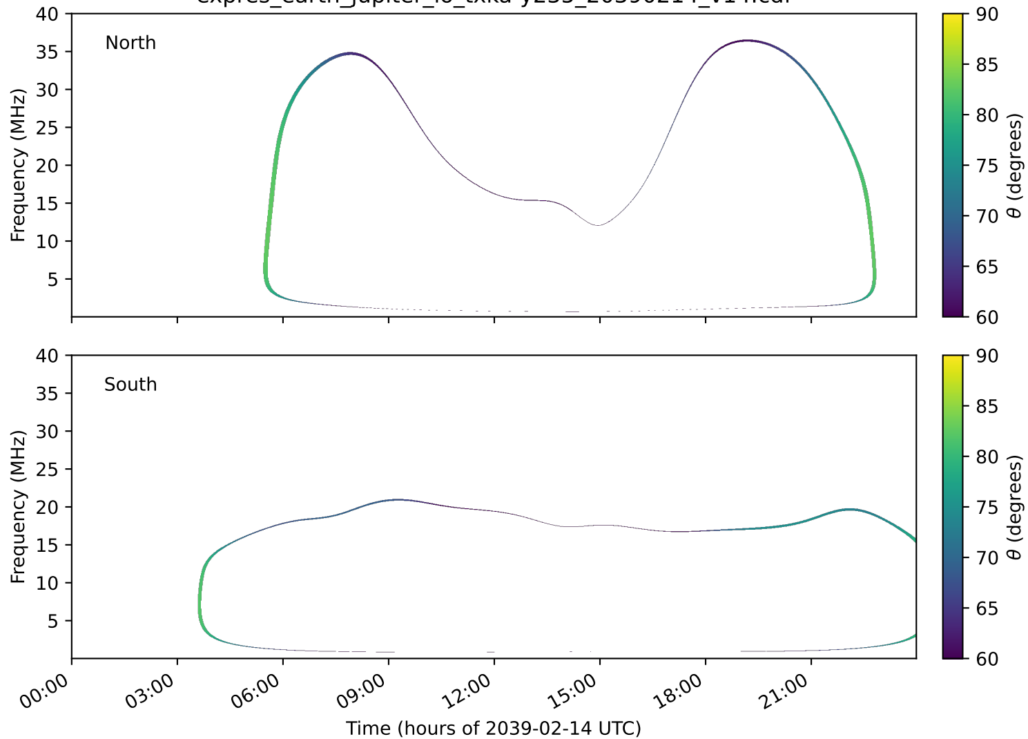
expres_earth_jupiter_io_txka-y235_20390214_v14.cdf
