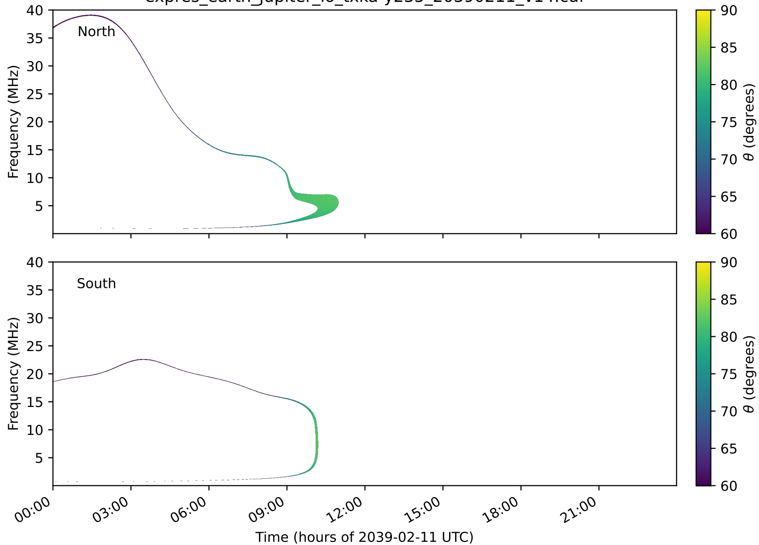
expres_earth_jupiter_io_txka-y235_20390211_v14.cdf
