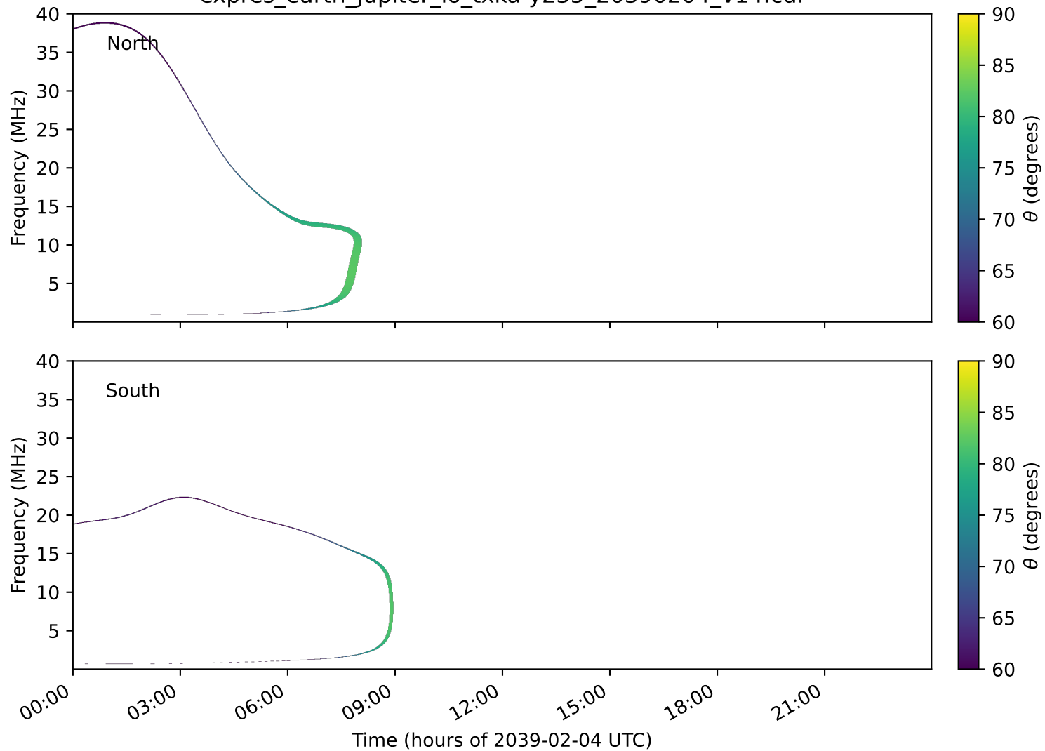
expres_earth_jupiter_io_txka-y235_20390204_v14.cdf
