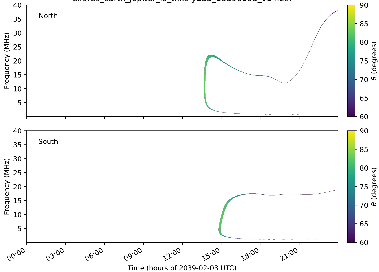
expres_earth_jupiter_io_txka-y235_20390203_v14.cdf
