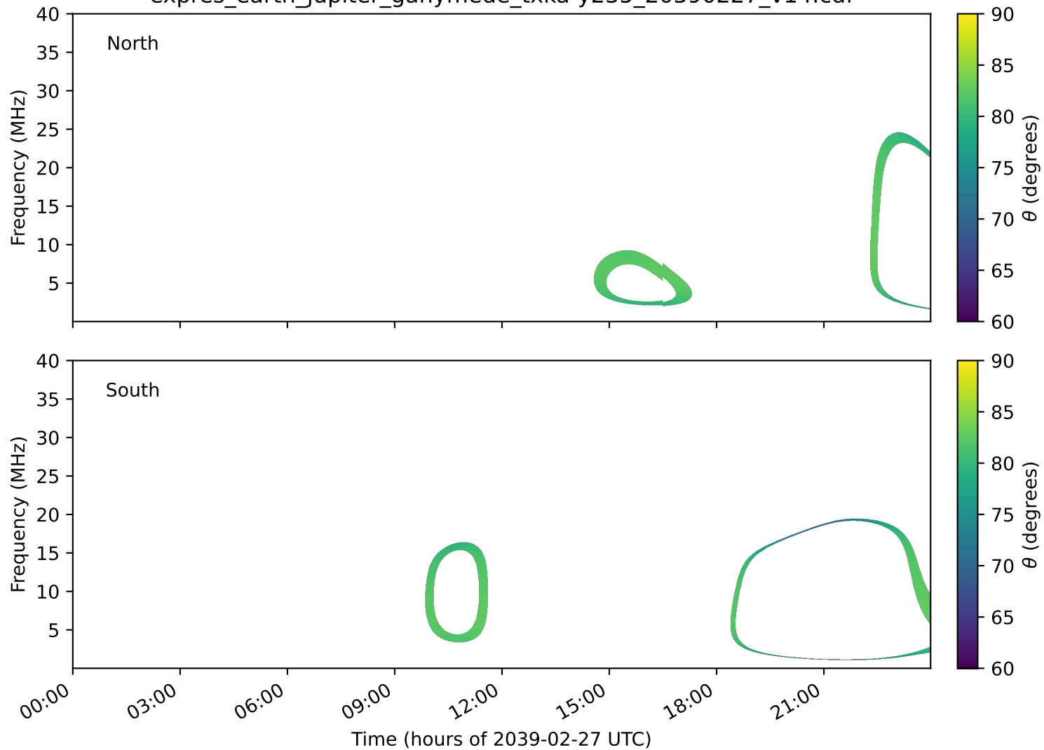
expres_earth_jupiter_ganymede_txka-y235_20390227_v14.cdf
