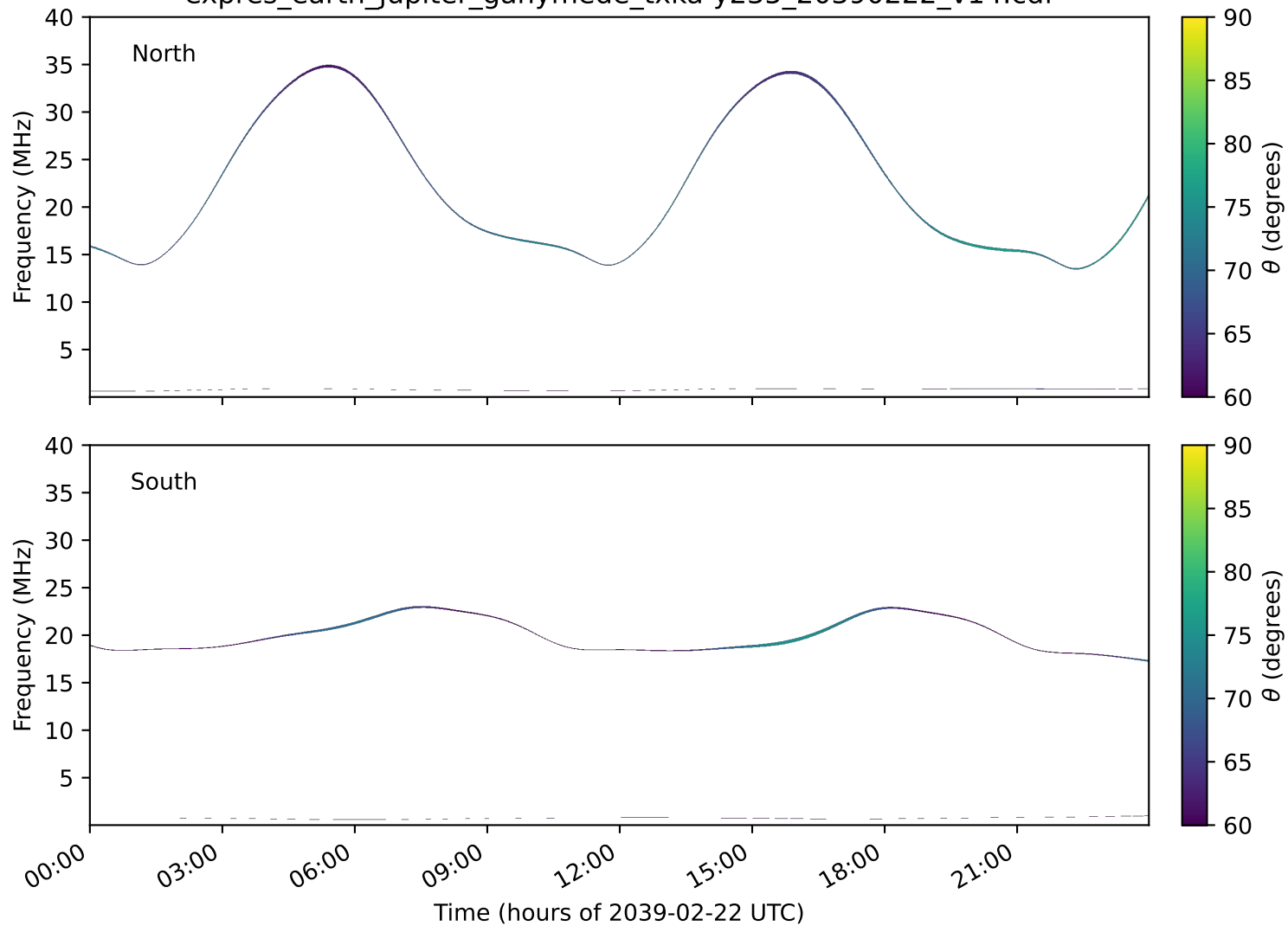
expres_earth_jupiter_ganymede_txka-y235_20390222_v14.cdf
