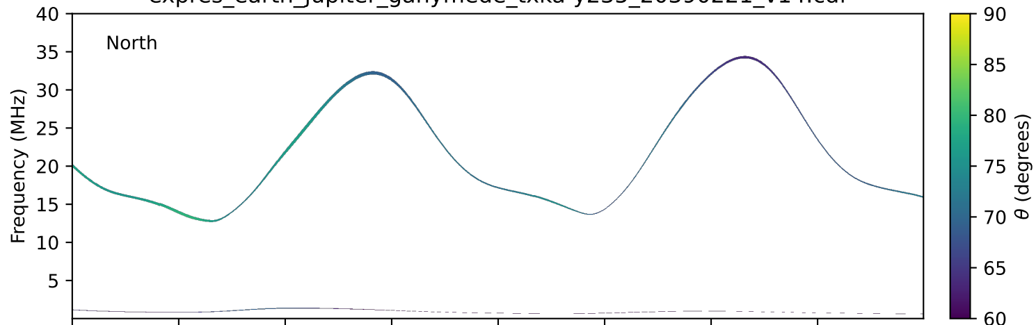
expres_earth_jupiter_ganymede_txka-y235_20390221_v14.cdf
