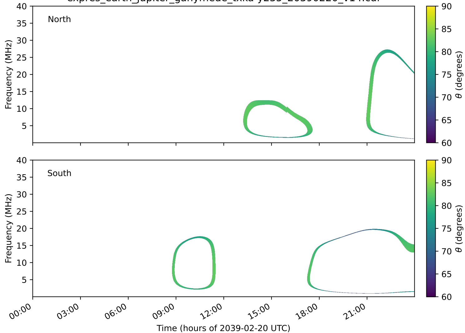
expres_earth_jupiter_ganymede_txka-y235_20390220_v14.cdf
