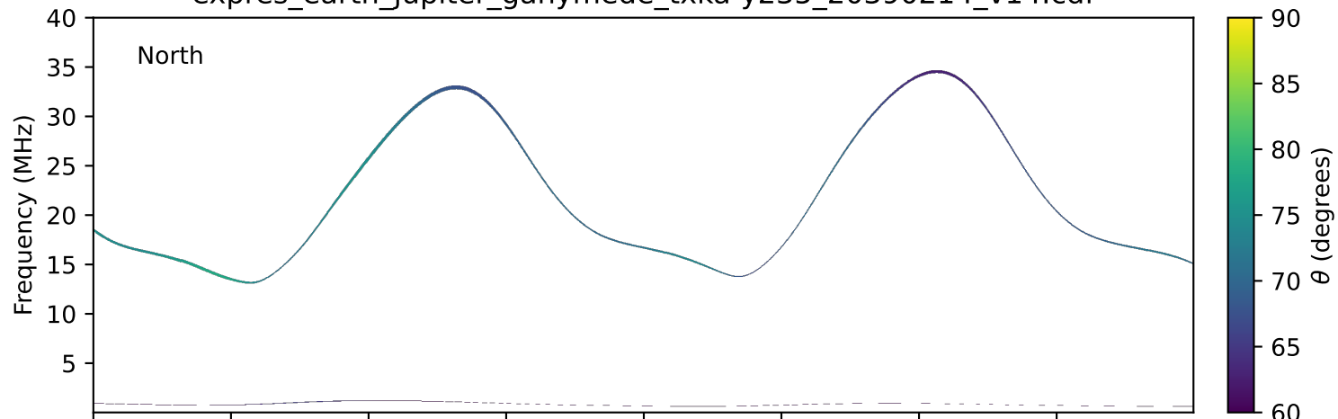
expres_earth_jupiter_ganymede_txka-y235_20390214_v14.cdf
