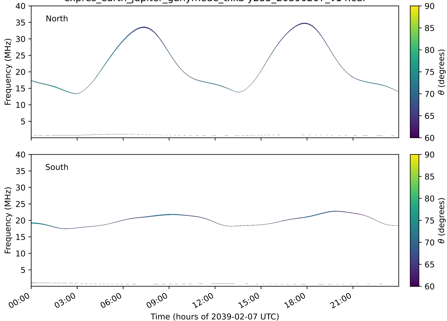
expres_earth_jupiter_ganymede_txka-y235_20390207_v14.cdf
