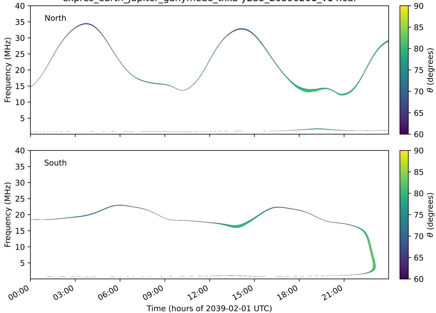
expres_earth_jupiter_ganymede_txka-y235_20390201_v14.cdf
