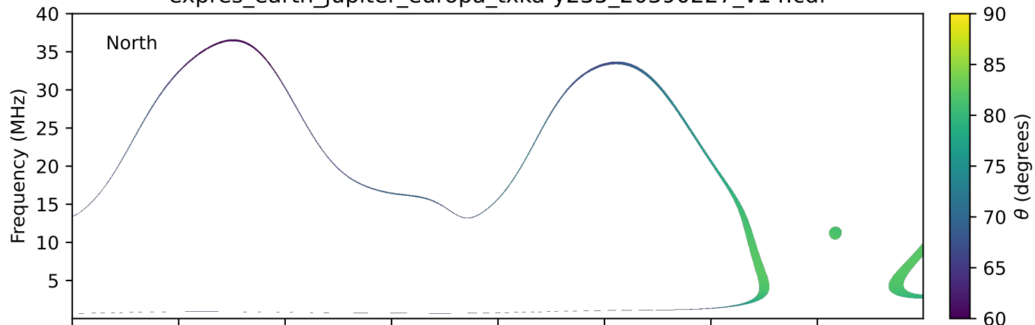
expres_earth_jupiter_europa_txka-y235_20390227_v14.cdf
