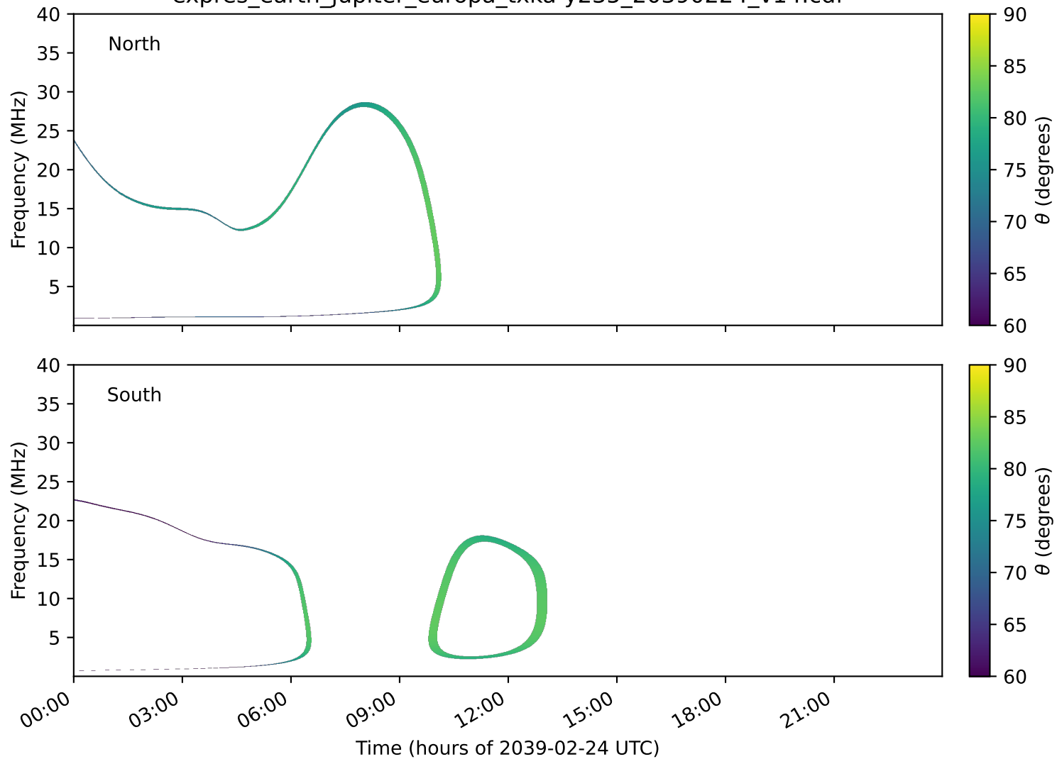
expres_earth_jupiter_europa_txka-y235_20390224_v14.cdf
