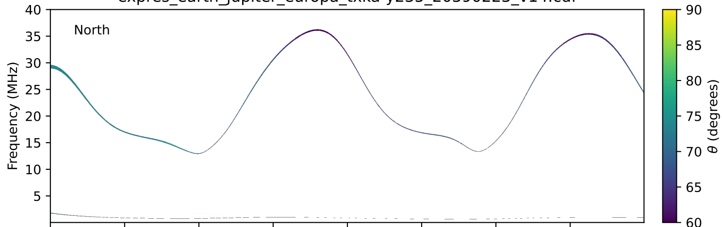
expres_earth_jupiter_europa_txka-y235_20390223_v14.cdf
