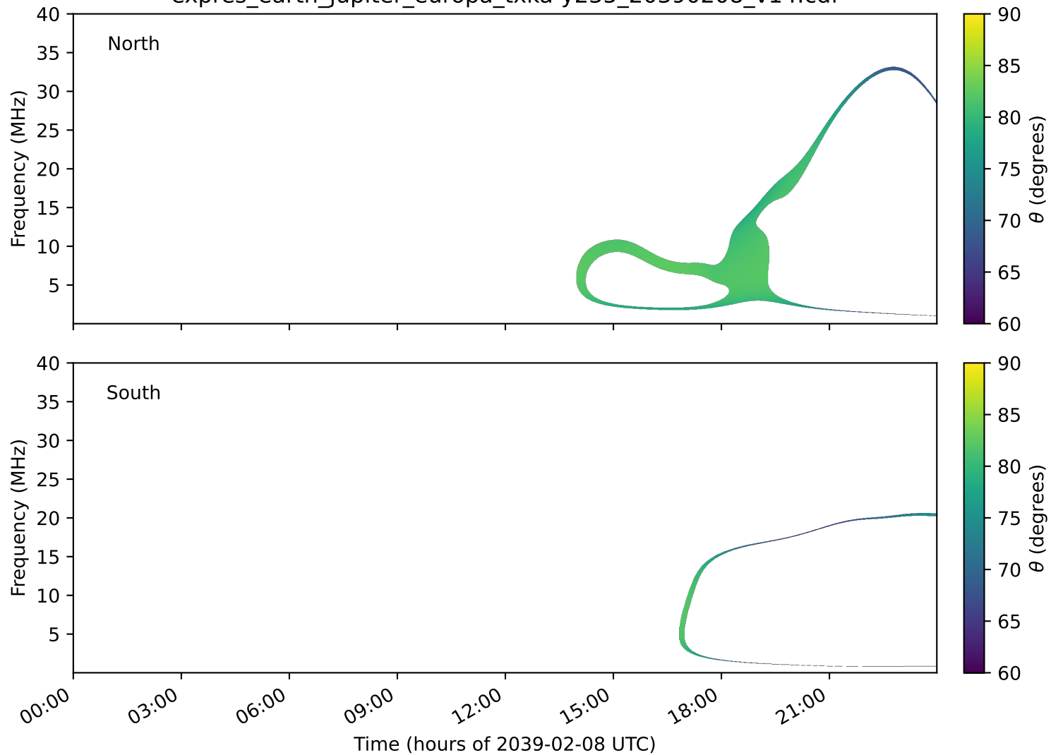
expres_earth_jupiter_europa_txka-y235_20390208_v14.cdf
