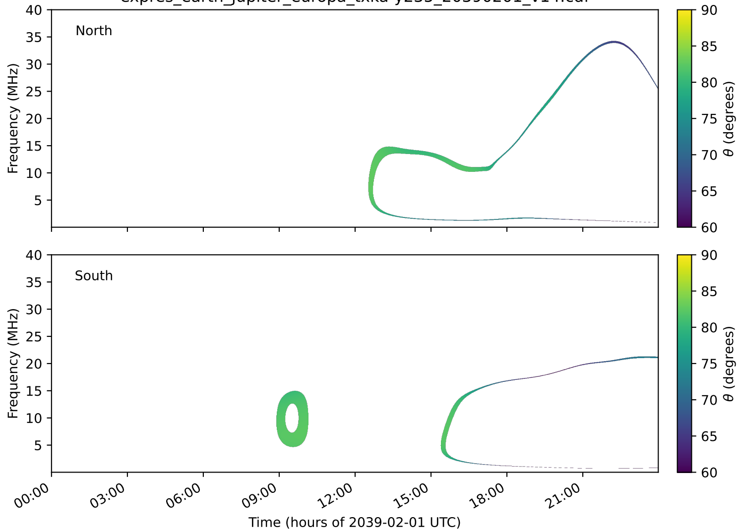
expres_earth_jupiter_europa_txka-y235_20390201_v14.cdf
