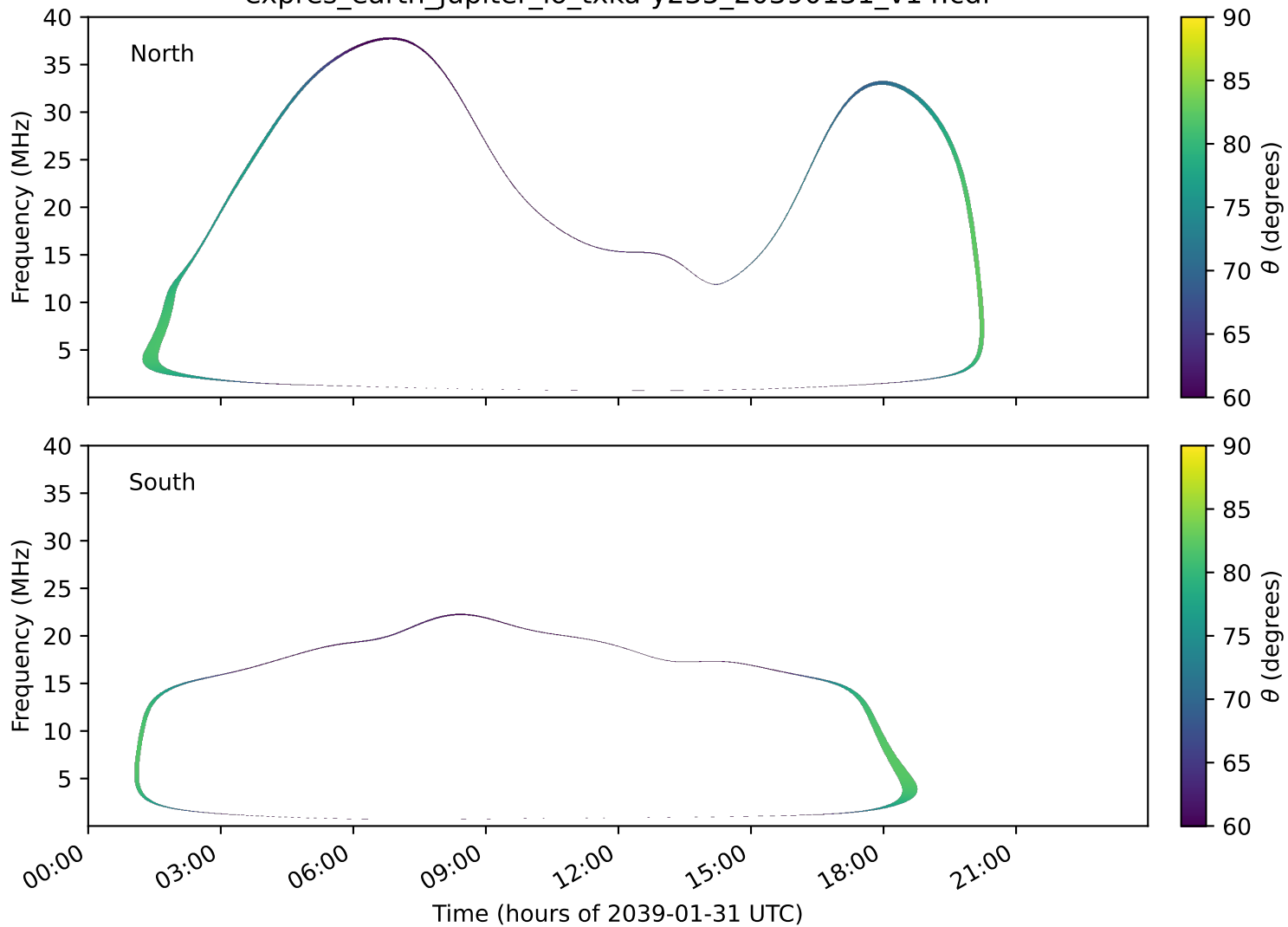
expres_earth_jupiter_io_txka-y235_20390131_v14.cdf
