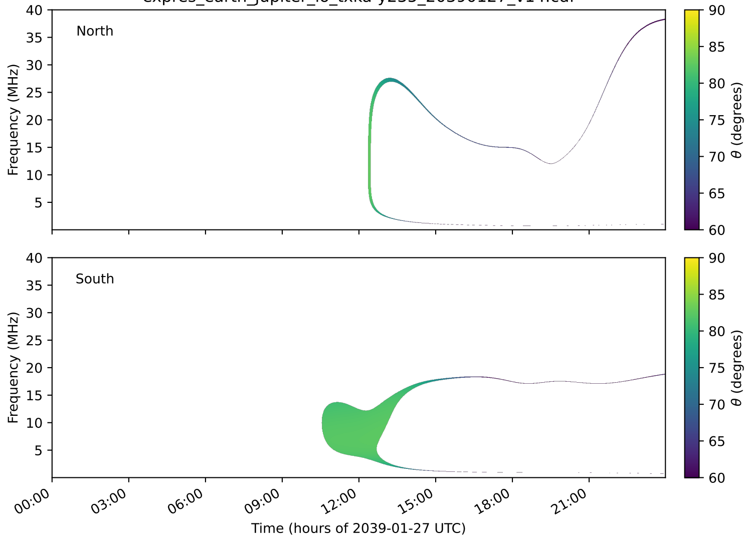
expres_earth_jupiter_io_txka-y235_20390127_v14.cdf
