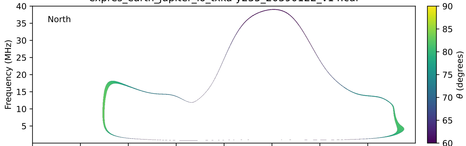
expres_earth_jupiter_io_txka-y235_20390122_v14.cdf
