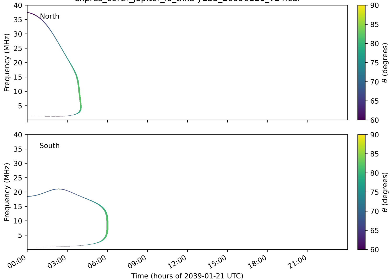
expres_earth_jupiter_io_txka-y235_20390121_v14.cdf
