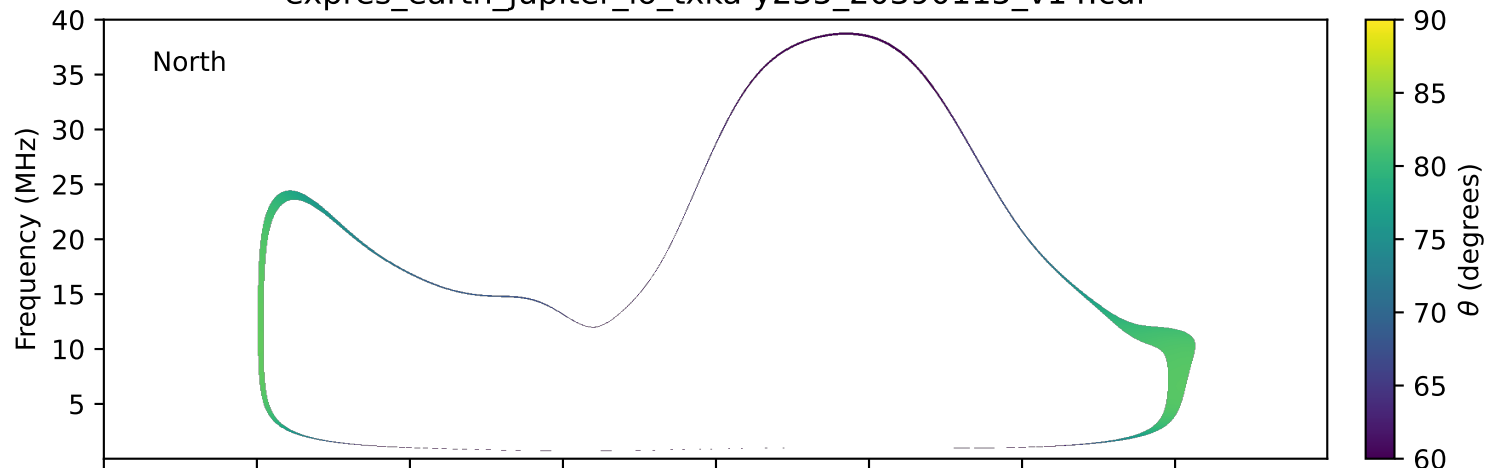
expres_earth_jupiter_io_txka-y235_20390115_v14.cdf
