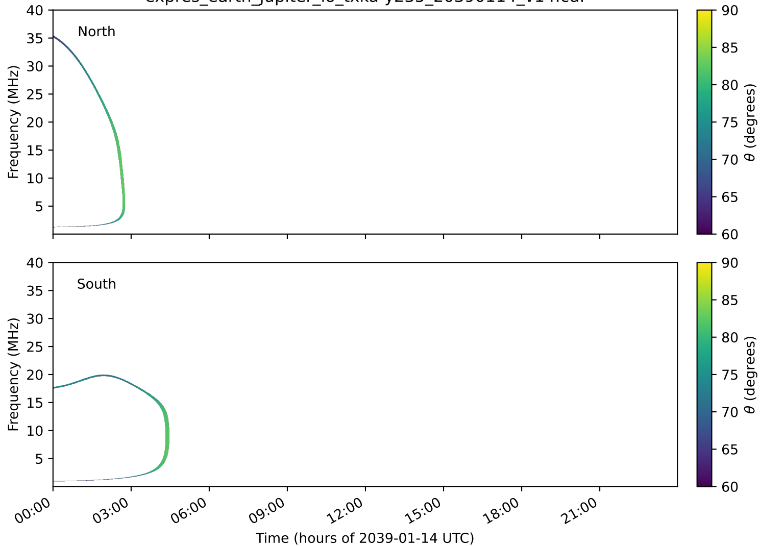
expres_earth_jupiter_io_txka-y235_20390114_v14.cdf
