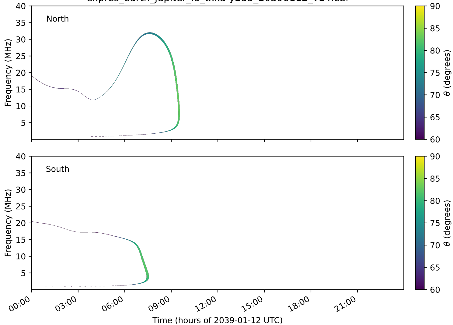
expres_earth_jupiter_io_txka-y235_20390112_v14.cdf
