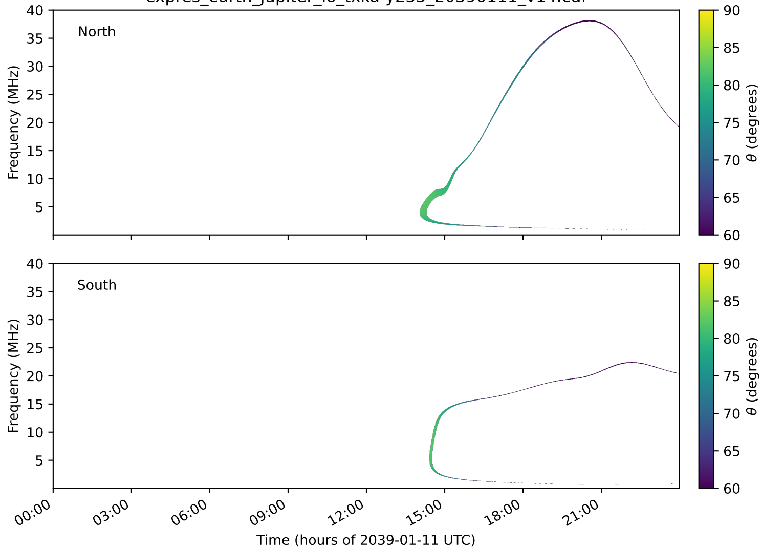
expres_earth_jupiter_io_txka-y235_20390111_v14.cdf
