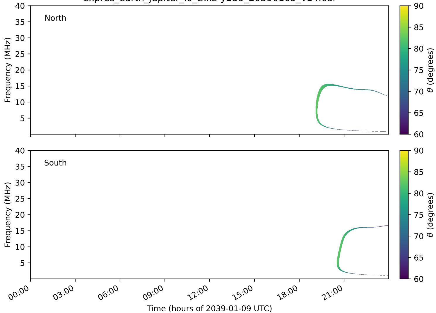
expres_earth_jupiter_io_txka-y235_20390109_v14.cdf
