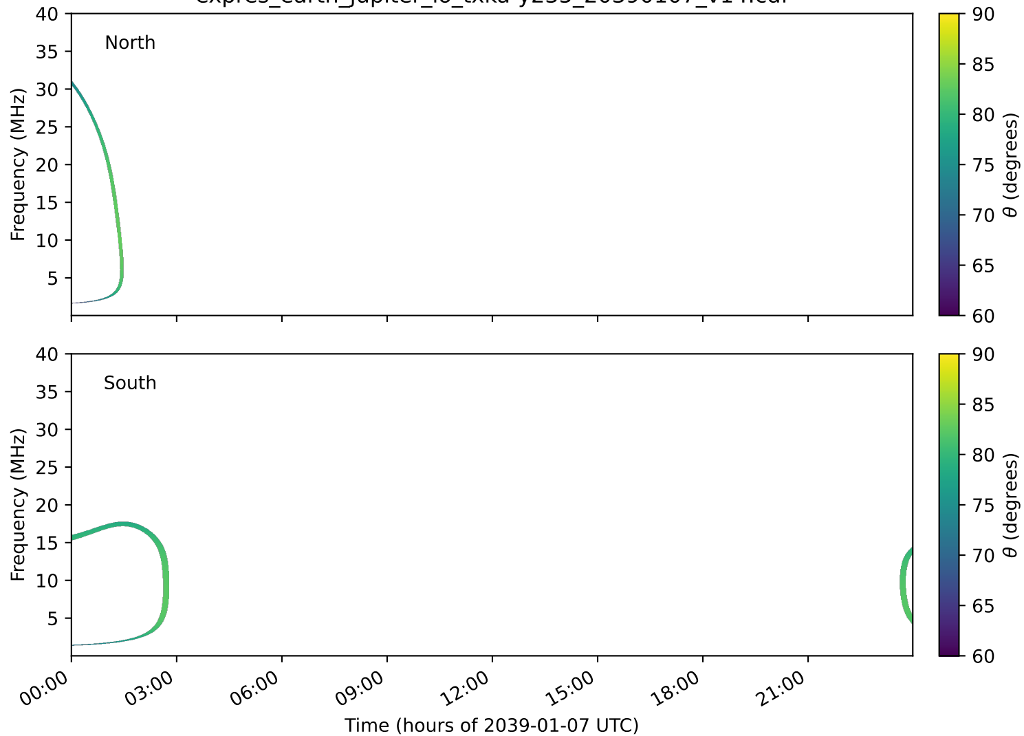
expres_earth_jupiter_io_txka-y235_20390107_v14.cdf
