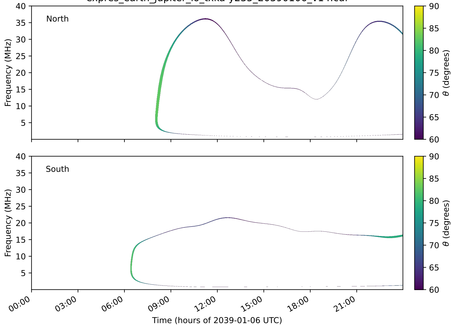
expres_earth_jupiter_io_txka-y235_20390106_v14.cdf
