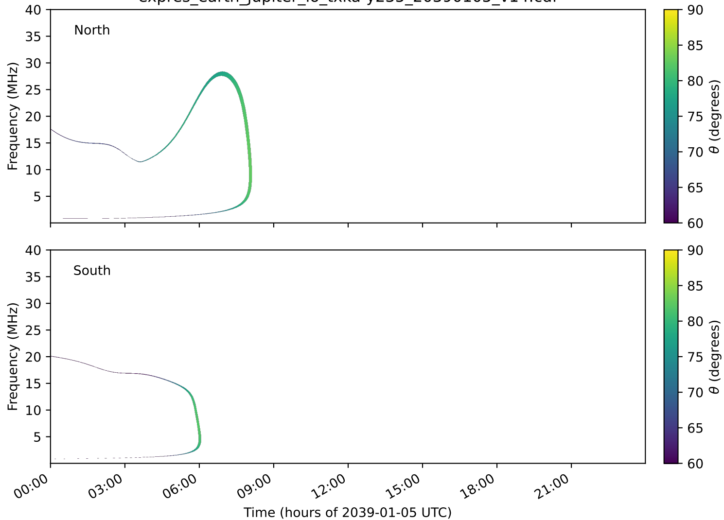
expres_earth_jupiter_io_txka-y235_20390105_v14.cdf
