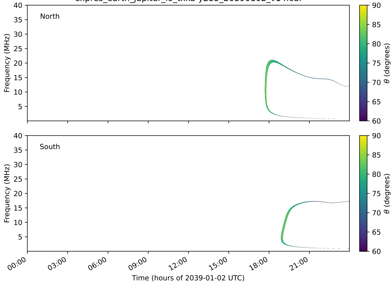
expres_earth_jupiter_io_txka-y235_20390102_v14.cdf
