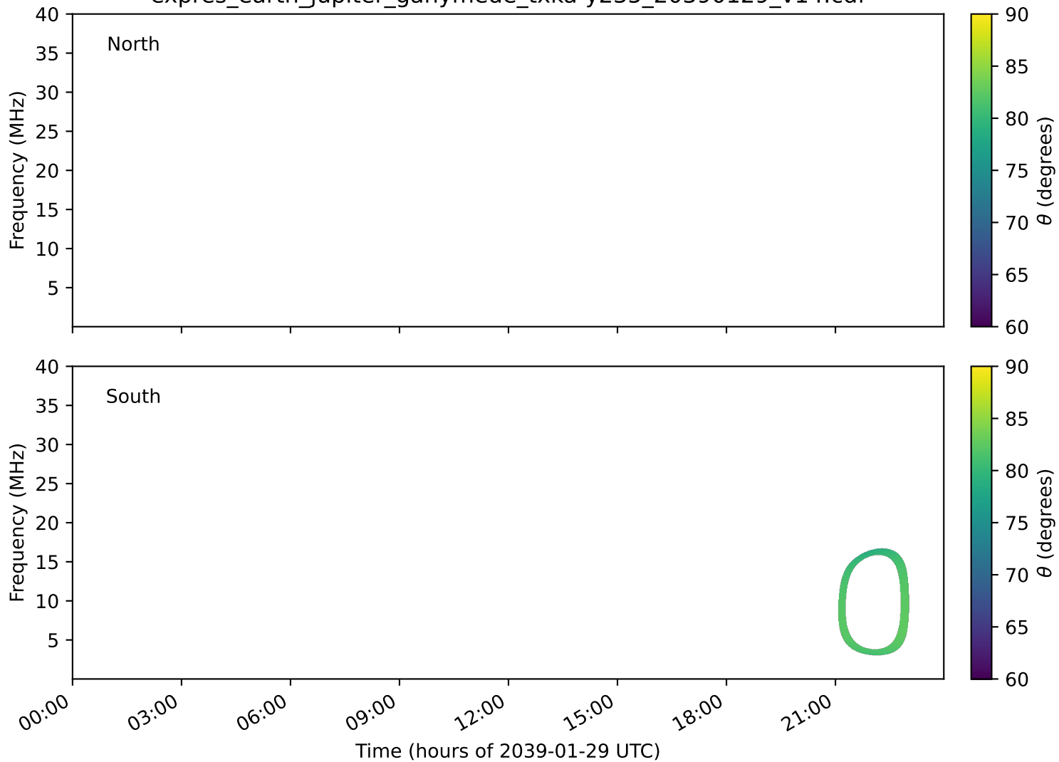
expres_earth_jupiter_ganymede_txka-y235_20390129_v14.cdf
