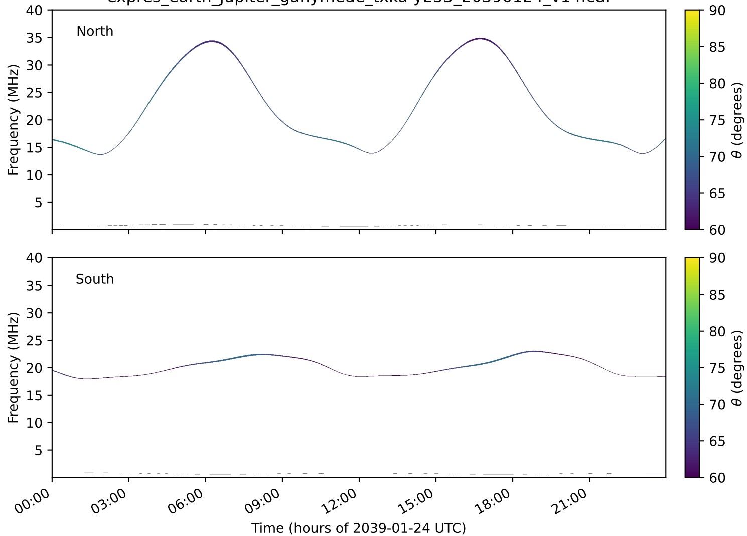
expres_earth_jupiter_ganymede_txka-y235_20390124_v14.cdf
