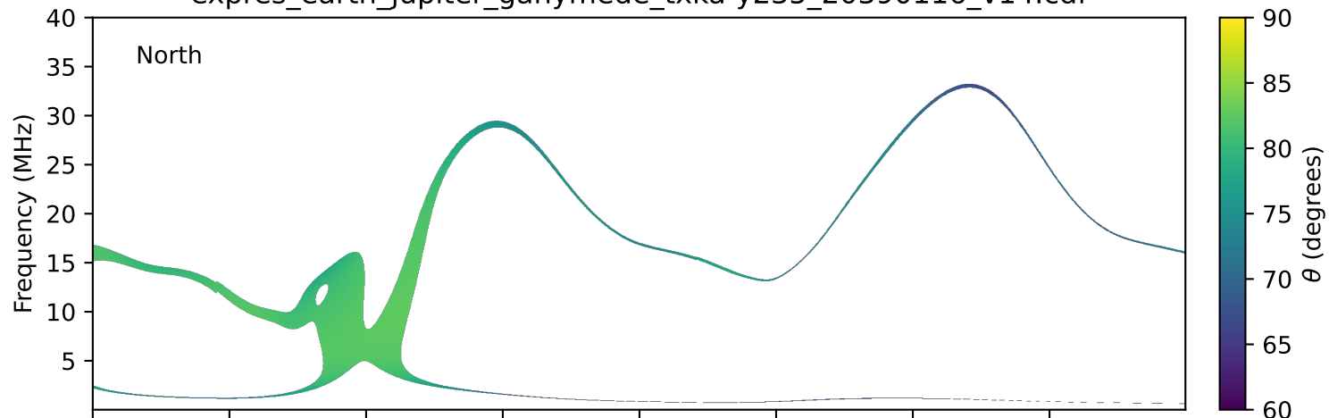
expres_earth_jupiter_ganymede_txka-y235_20390116_v14.cdf
