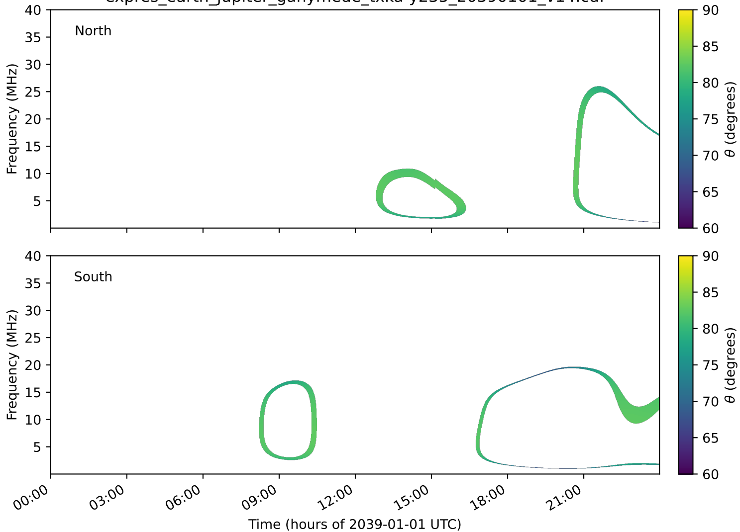
expres_earth_jupiter_ganymede_txka-y235_20390101_v14.cdf
