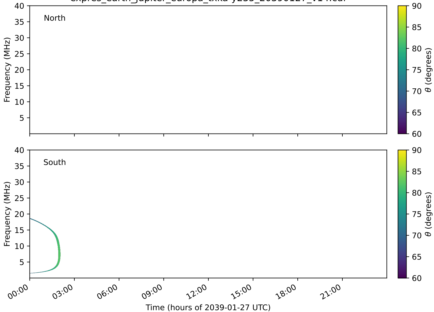
expres_earth_jupiter_europa_txka-y235_20390127_v14.cdf
