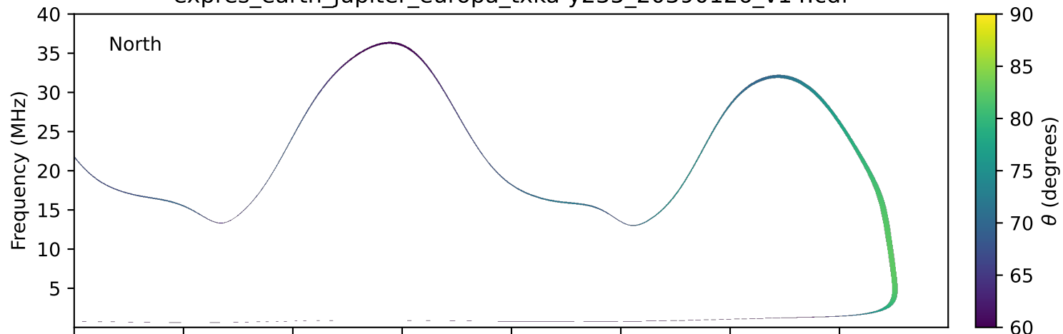
expres_earth_jupiter_europa_txka-y235_20390126_v14.cdf
