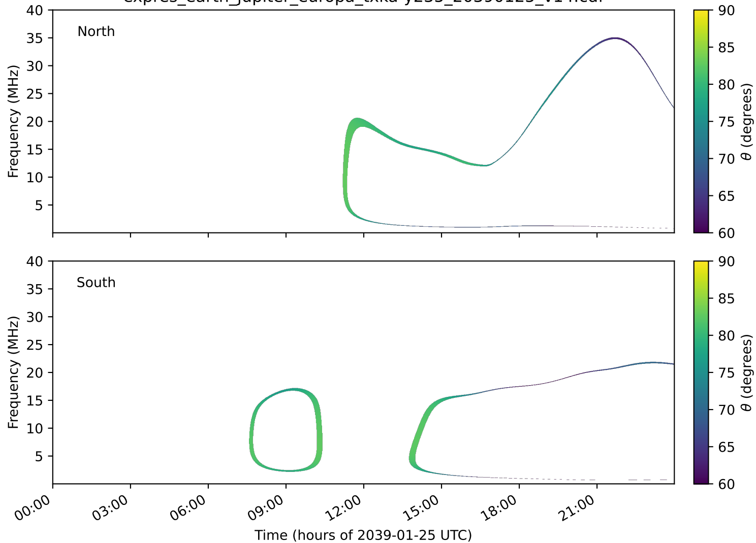
expres_earth_jupiter_europa_txka-y235_20390125_v14.cdf
