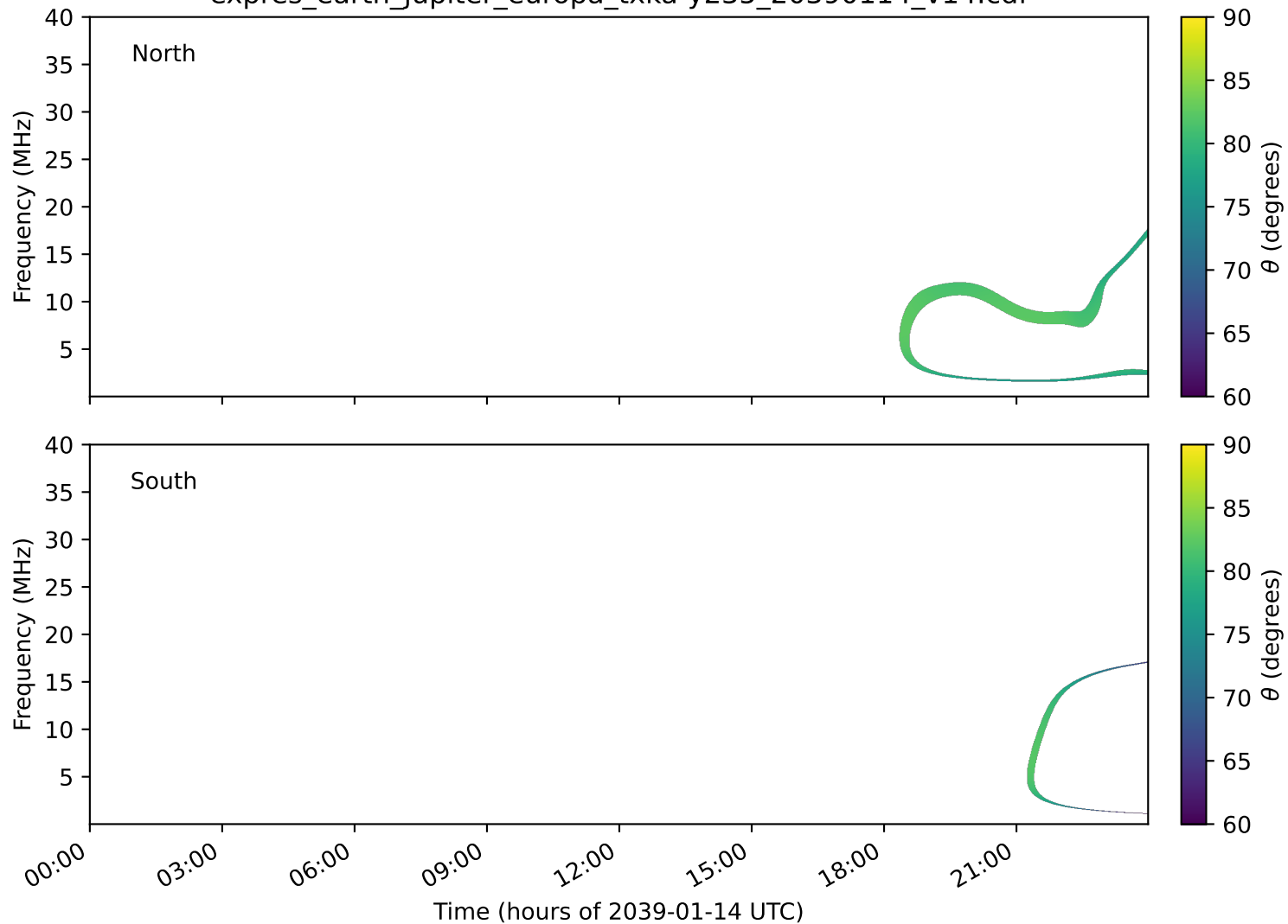
expres_earth_jupiter_europa_txka-y235_20390114_v14.cdf
