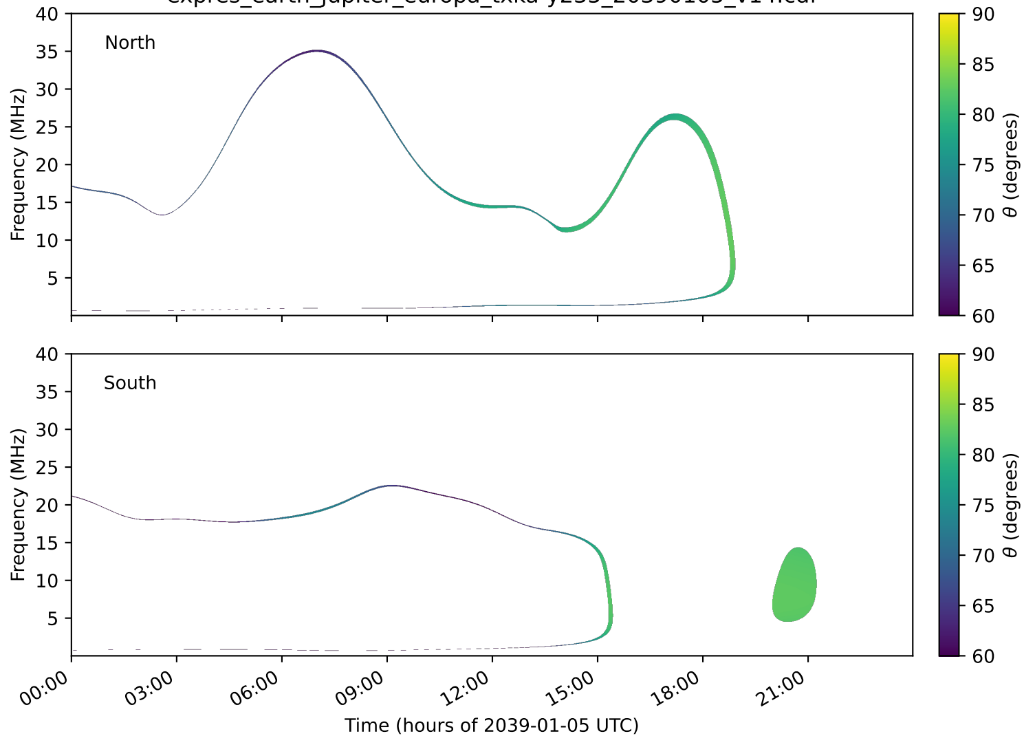
expres_earth_jupiter_europa_txka-y235_20390105_v14.cdf
