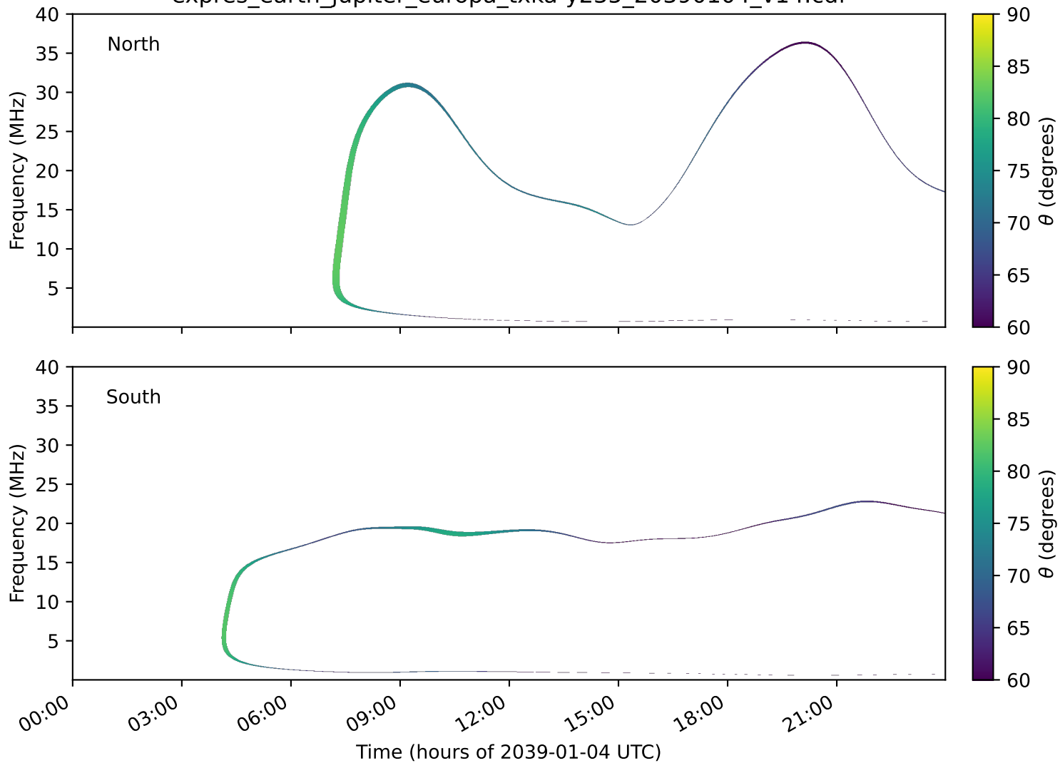
expres_earth_jupiter_europa_txka-y235_20390104_v14.cdf
