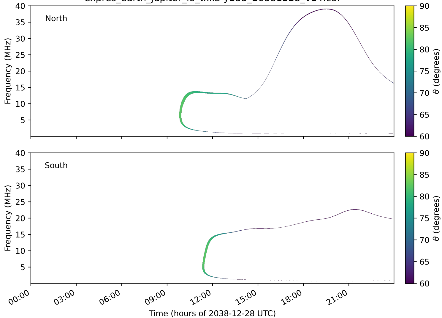
expres_earth_jupiter_io_txka-y235_20381228_v14.cdf
