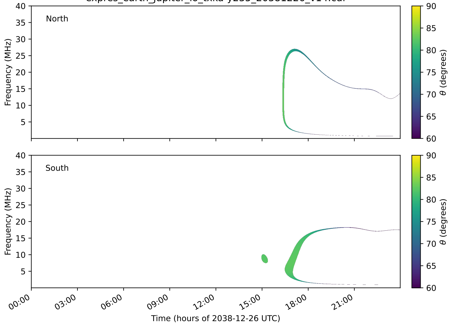
expres_earth_jupiter_io_txka-y235_20381226_v14.cdf
