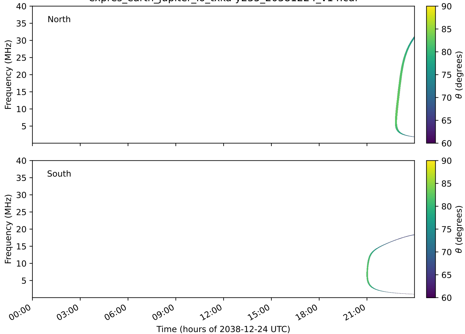
expres_earth_jupiter_io_txka-y235_20381224_v14.cdf
